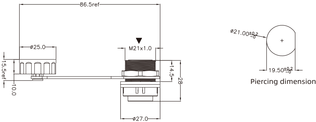
EW-RJ45 Plastic cable mount adapter socket
