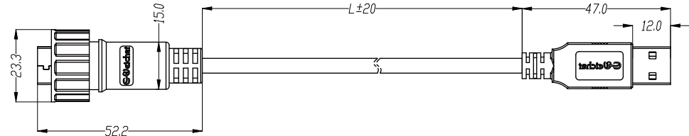
EU-USB Interlocked male plug
