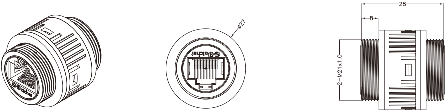
EW-RJ45 Plastic cable mount adapter socket
