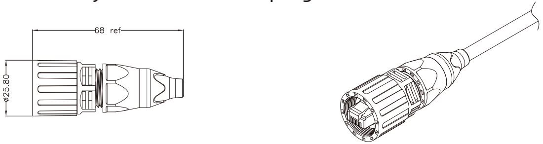
EW-RJ45 Threaded style - cable mount plug
