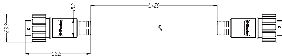
EU-USB Interlocked dual male plug
