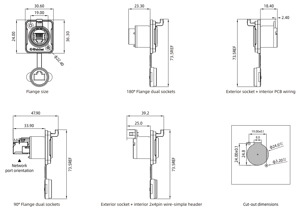
EW-RJ45 Snap-on style - flange mount socket
