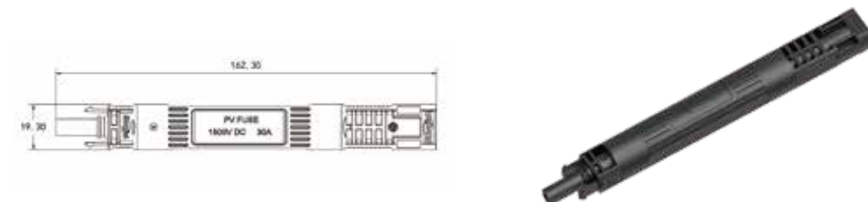
EW-PV4-XXXXXX PV4 fuse, 1500V DC/30A
