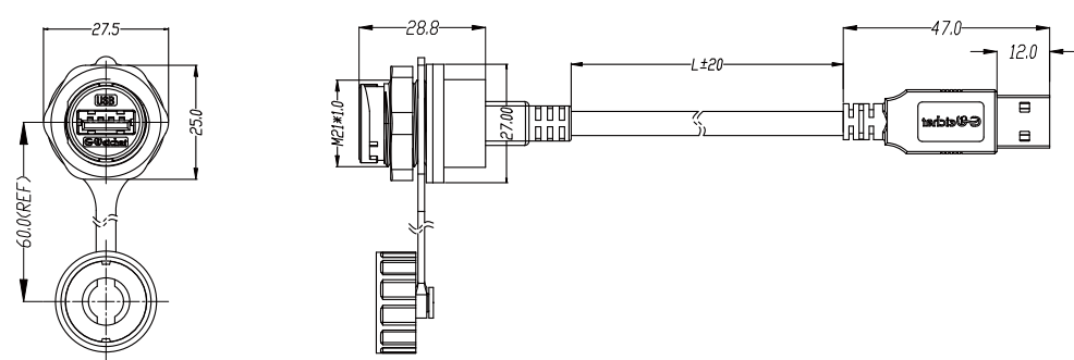
EU-USB Cable mount male and female
