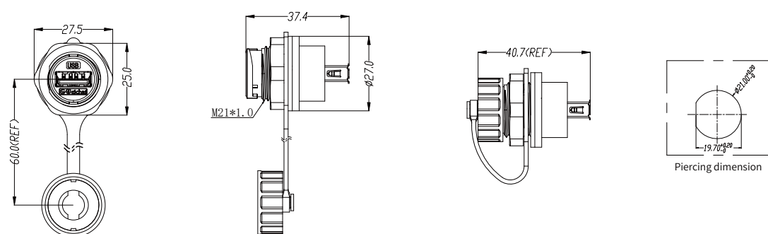
EU-Panel mount female
