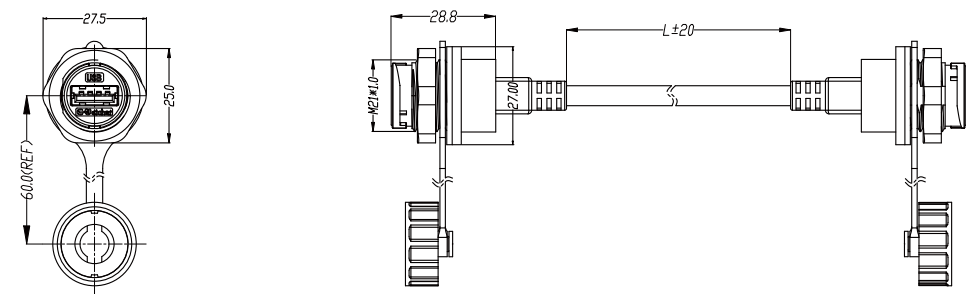
EU-USB Cable mount dual female
